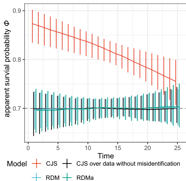
FIGURE 4 Survival probabilities estimated with both the CJS ( \Phi_T p ), the RDM and RDMa models ( \Phi_T p, \Theta ) using the simulation scenario \Phi, p, \Theta , \Phi = 0.7 , p = 0.9 , \Theta = 0.95 , 25 individuals marked every occasion). In contrast to the CJS (red lines), the temporal trends in survival probabilities estimated by the RDM (blue) and RDMa (green) models were correctly estimated not to be different from zero, which is also illustrated by their almost identical estimates to those from the CJS model ran for the same data before misidentifications were introduced (black lines)
